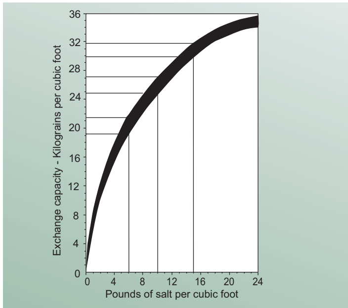
Fig. 1 Exchange capacity vs. regeneration level Sodium form C-800x10 LT UPS Cation Resin
