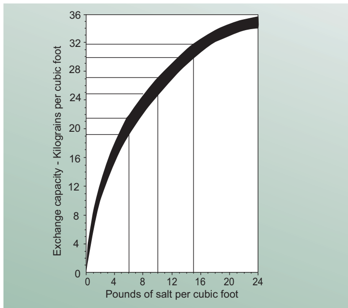
Fig. 1 Exchange capacity vs. regeneration level Sodium form C-800x10 Cation Resin
